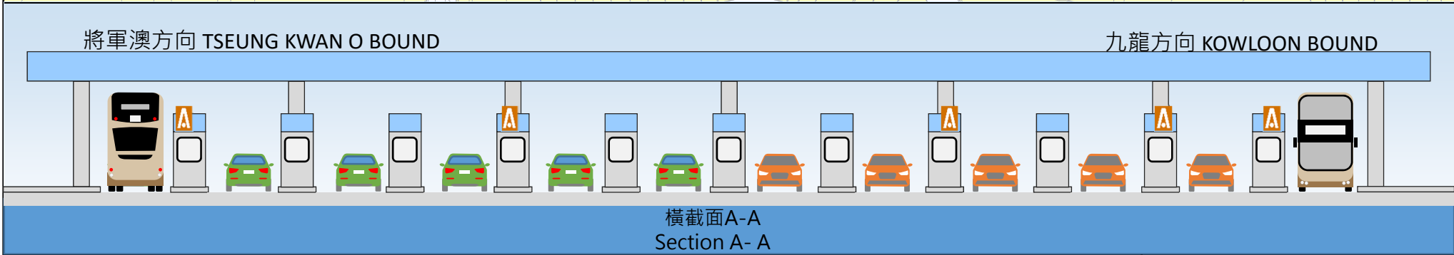
將軍澳隧道收費廣場現時的交通安排 EXISTING TRAFFIC ARRANGEMENT AT TSEUNG KWAN O TUNNEL TOLL PLAZA
